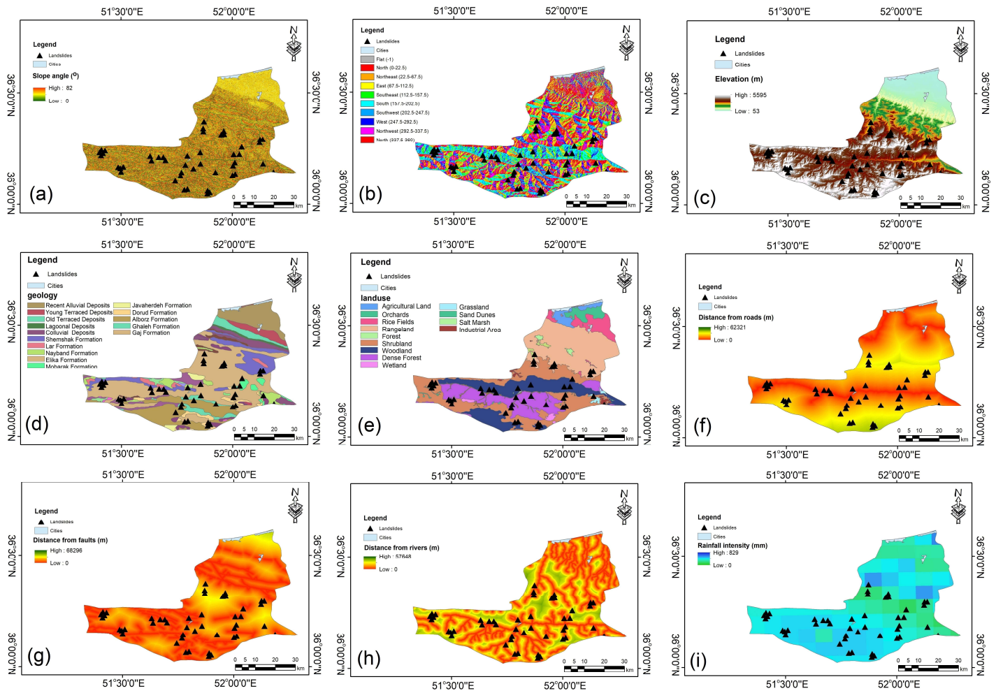
Fig. 3 Triggering factor index maps: (a) slope angle, (b) aspect, (c) elevation, (d) lithology, (e) land use, (f) distance from roads, (g) distance from faults, (h) distance from rivers, (i) rainfall intensity
